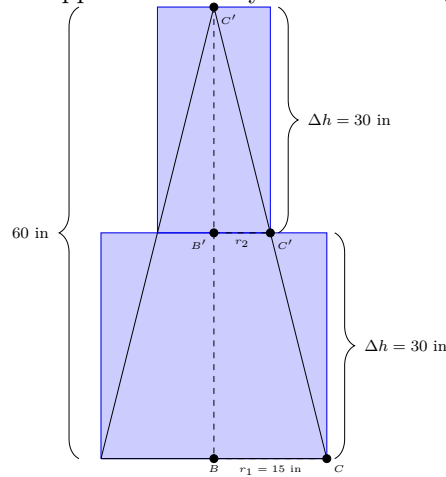
Figure 139 15× 60 cylindrical cone sliced into two pieces.
