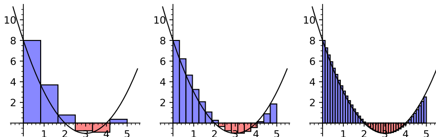
Figure 100 Improving approximations of \int_0^5 (x-2)(x-4) dx
