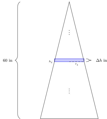
Figure 142 15× 60 cylindrical cone sliced into many pieces.
