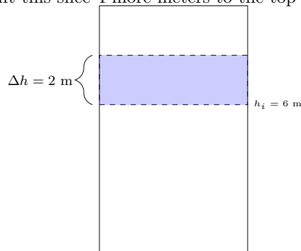
Figure 155 2m thick slice of water lifted 4m.
