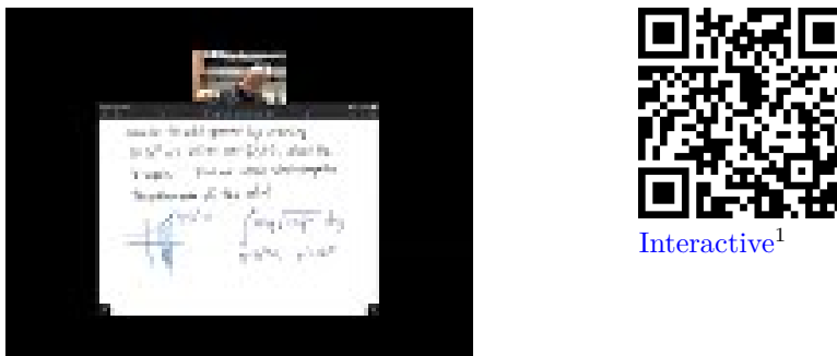
Figure 135 Video: Compute surface areas of surfaces of revolution
