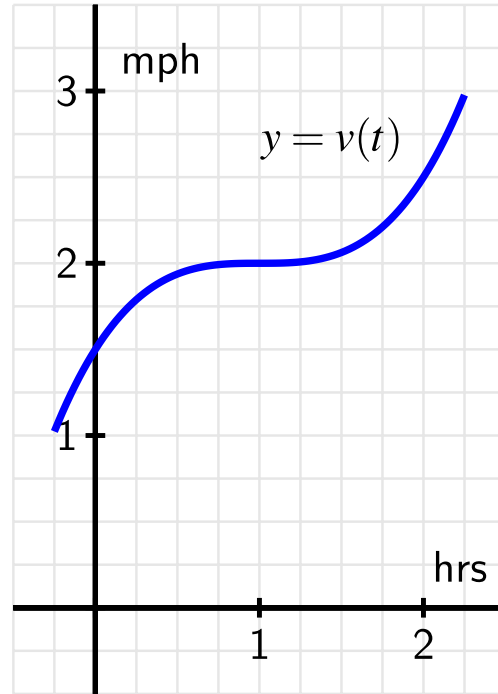
Figure 60 The graph of y = v(t) .
