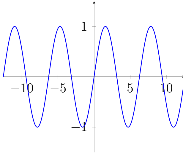
Figure 26 A mysterious periodic function.
